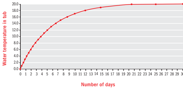
Calculated thermal conduction for 400L PUR insulated tub filled with 0°C water and T environment = 20°C
